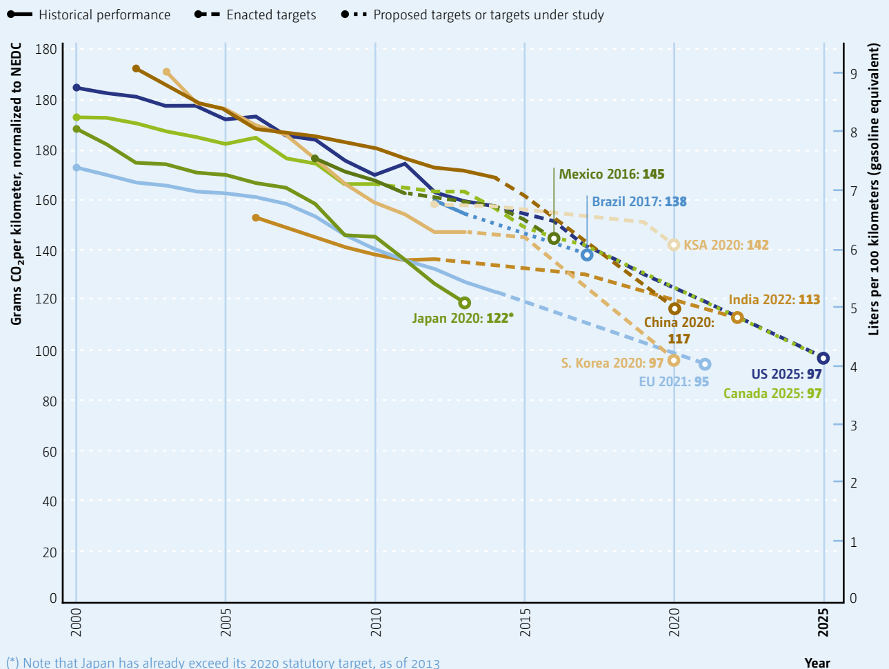
Figure 21 Passenger car sales CO 2 emission targets and sales weighted averaged actual fleet historical performance (ICCT, 2016)
